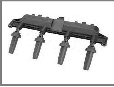
Ateşleme Bobini Ignition Coil SAXO-XSARA-106-206-306 1.4 1.6i 1.6V
