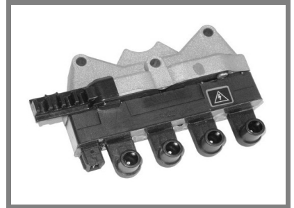
Ateşleme Bobini Ignition Coil DOBLO-ALBEA-PALİO-MAREA-BRAVA- BRAVO-SIENA 1.6 16V
