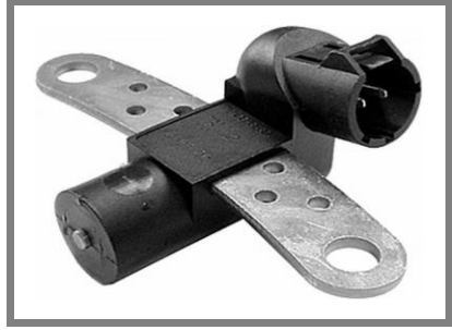
Krank Devir (Volan) Sensörü Sensor, Crankshaft Pulse CLIO II-KANGOO 1.5 dCi
