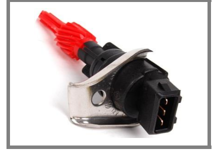
Hız (KM) Sensörü Sensor, Odometer A3-BORA-GOLF IV 1.6-A3 1.8 GOLF 1.8- GOLF IV 1.9TDI
