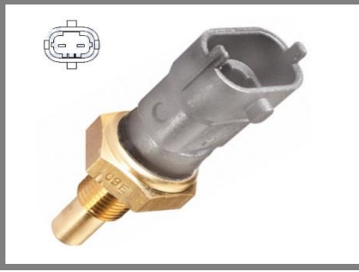
Hararet Müşürü Water Temperature Sensor VECTRA B 1.8i 2.0i 16V
